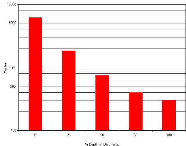
AGM Cycle Life vs. Depth of Discharge at +25°C (77°F) Based on BCI 2-hour Capacity
