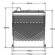
ODP-AGM34 LEFT POSITIVE SAE TERMINALS
