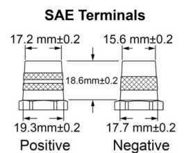
ODP-AGM65 LEFT POSITIVE SAE TERMINALS
