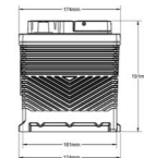
ODP-AGM94R/H7/L4 RIGHT POSITIVE SAE TERMINALS
