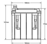
ODS-AGM70A RIGHT POSITIVE SAE TERMINALS
