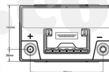
ODX-AGM65 LEFT POSITIVE SAE TERMINALS
