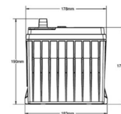
ODX-AGM65 LEFT POSITIVE SAE TERMINALS
