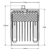
ODP-AGM31A LEFT POSITIVE SAE TERMINALS
