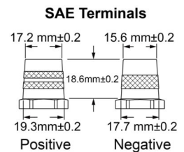
ODP-AGM31A LEFT POSITIVE SAE TERMINALS
