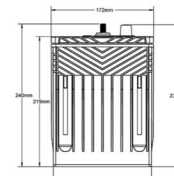
ODP-AGM31M RIGHT POSITIVE DUAL TERMINALS (SAE & STUD)
