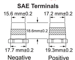
ODP-AGM34R RIGHT POSITIVE SAE TERMINALS
