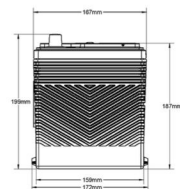
ODP-AGM34R RIGHT POSITIVE SAE TERMINALS
