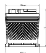
ODP-AGM48/H6/L3 RIGHT POSITIVE SAE TERMINALS
