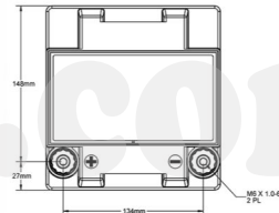
ODS-AGM28 LEFT POSITIVE FEMALE TERMINALS
