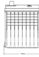
ODP-AGM25 LEFT POSITIVE SAE TERMINALS
