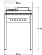
ODS-AGM15LMJ RIGHT POSITIVE FEMALE TERMINAL
