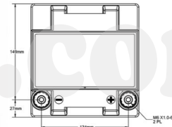
ODS-AGM28L RIGHT POSITIVE FEMALE TERMINAL
