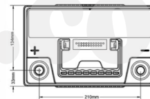
ODX-AGM34 LEFT POSITIVE SAE TERMINALS
