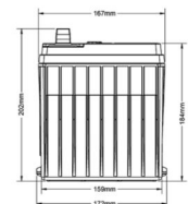
ODX-AGM34 LEFT POSITIVE SAE TERMINALS
