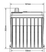
ODX-AGM34 LEFT POSITIVE SAE TERMINALS
