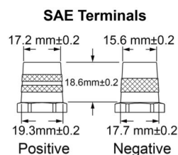
ODP-AGM25 LEFT POSITIVE SAE TERMINALS
