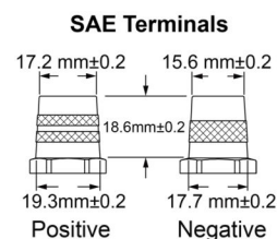
ODP-AGM31A LEFT POSITIVE SAE TERMINALS
