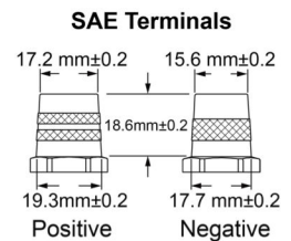
ODP-AGM35 RIGHT POSITIVE SAE TERMINALS
