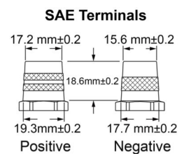
ODP-AGM65 LEFT POSITIVE SAE TERMINALS
