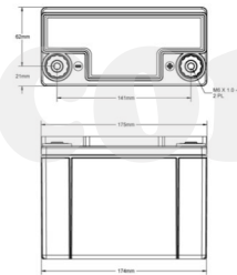
ODS-AGM15L RIGHT POSITIVE FEMALE TERMINAL
