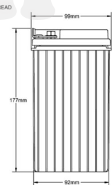
ODS-AGM16CL RIGHT POSITIVE FRONT FEMALE CONNECTION
