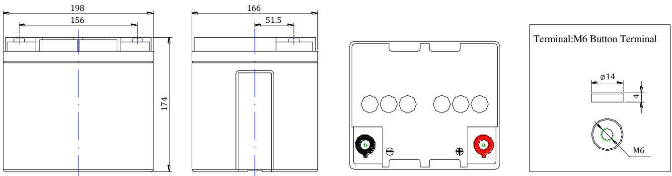
Battery bank spacing required 12.5mm (1/2"inch) minimum
