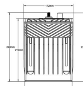
ODP-AGM31M RIGHT POSITIVE DUAL TERMINALS (SAE & STUD)
