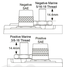
ODP-AGM34M LEFT POSITIVE DUAL TERMINALS (SAE & STUD)
