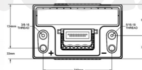
ODP-AGM34M LEFT POSITIVE DUAL TERMINALS (SAE & STUD)
