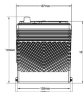
ODP-AGM34R RIGHT POSITIVE SAE TERMINALS
