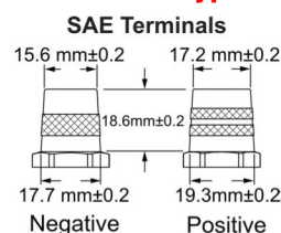
ODP-AGM34R RIGHT POSITIVE SAE TERMINALS
