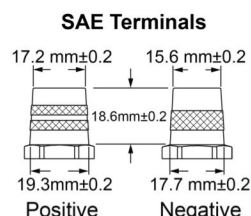
ODP-AGM35 RIGHT POSITIVE SAE TERMINALS
