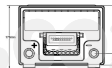
ODP-AGM75/86 LEFT POSITIVE DUAL TERMINALS (SAE & SIDE)
